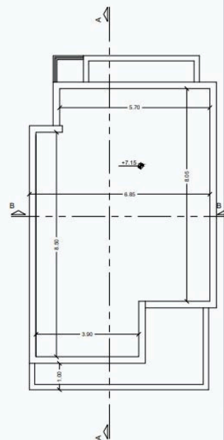
Roof Plan
