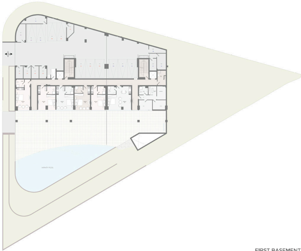
FIRST BASEMENT PLAN
