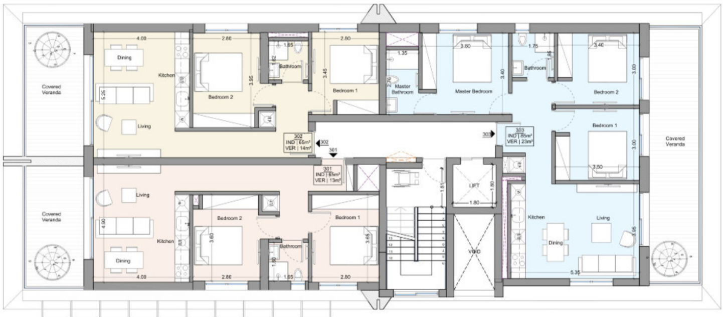
3rdFloor
