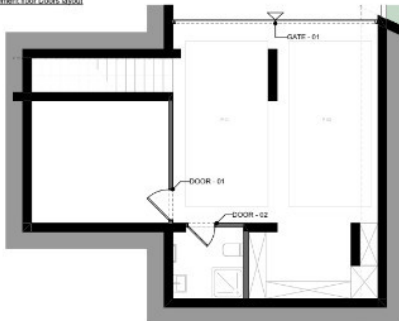
Basement floor Doors layout
