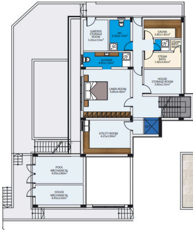
Basement Plan
