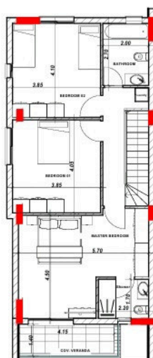
FIRST FLOOR
