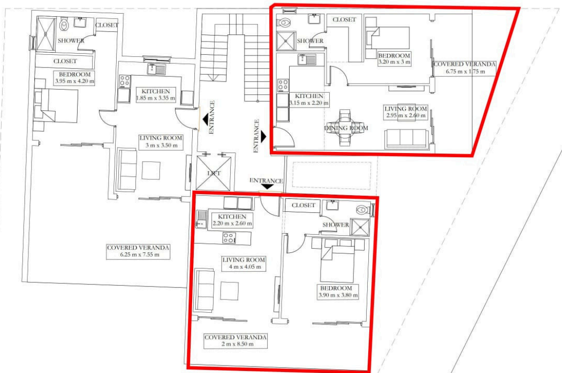
1 FIRST FLOOR PLAN NTS
