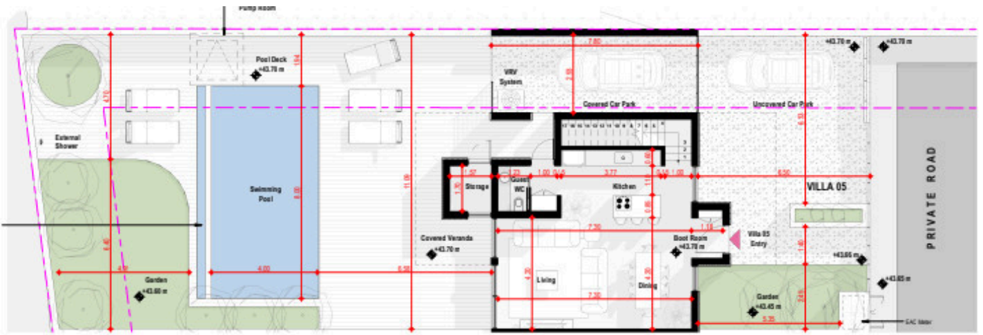
1 Ground Floor Plan - Villa 05 1 : 100
