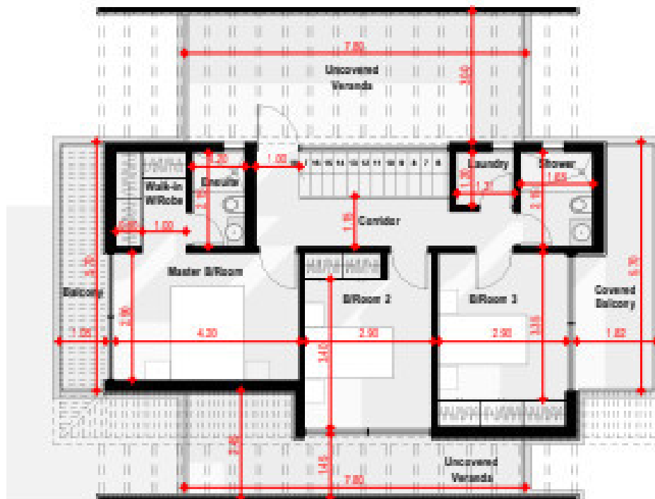
2 First Floor Plan - Villa 04 1 : 100
