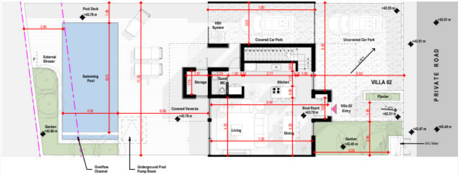
1 Ground Floor Plan - Villa 02 1 : 100
