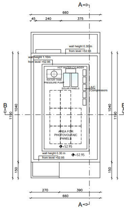
ROOF PLAN (AREA FOR SOLAR AND PHOTOVOLTAIC PANELS)
