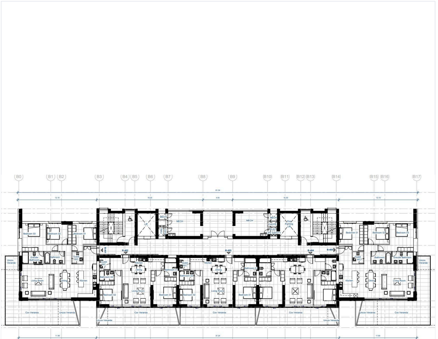
① 4th Floor 1-100 1:100
