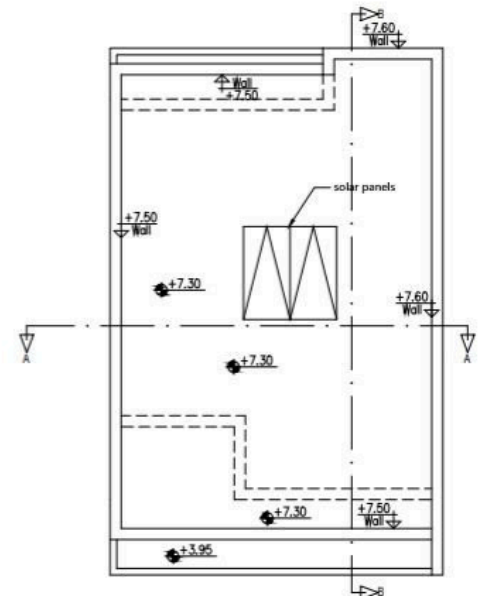
ROOF PLAN
