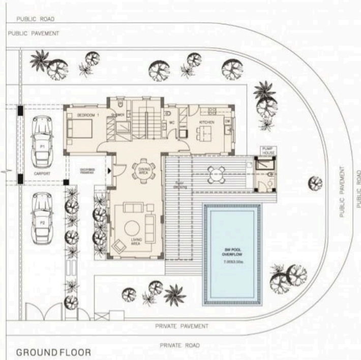
3 BEDROOM VILLA
