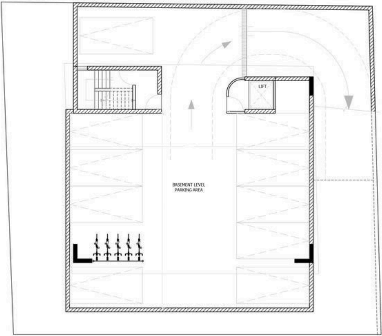
BASEMENT PLAN
