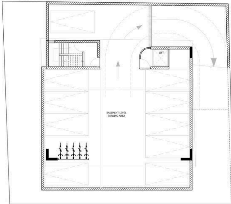
BASEMENT PLAN
